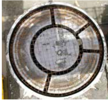
Inverted Mould with Reinforcing Ready for Concrete
